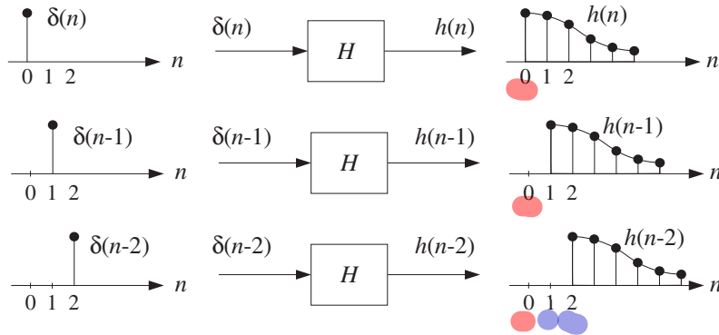
Fig. 3.3.2 Delayed impulse responses of an LTI system.
