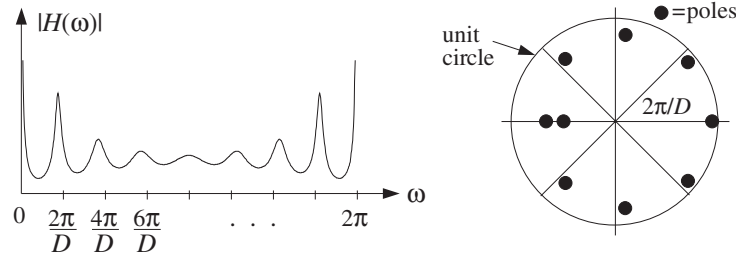
Fig. 8.2.24 Magnitude response of lowpass reverberator, for D = 8 .
