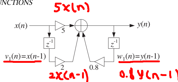
Fig. 6.2.1 Direct form realization of H(z) .
