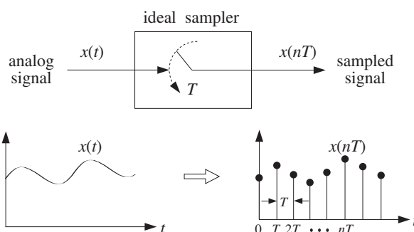
Fig. 1.3.1 Ideal sampler.
