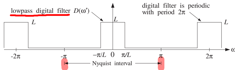
Fig. 12.2.3 Ideal lowpass digital filter operating at high rate Lf_s .
