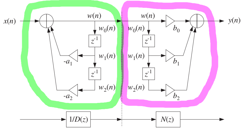
Fig. 7.2.2 Interchanging N(z) and 1/D(z) .
