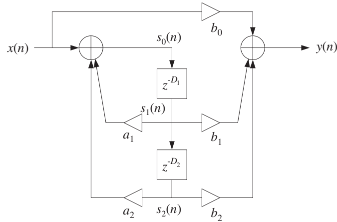
Fig. 8.2.29 Multitap delay effects processor.
