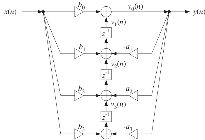
Fig. 7.7.1 Transpose of canonical realization.
