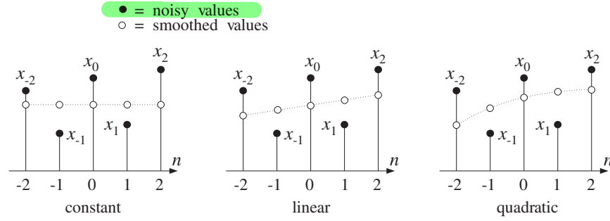
Fig. 8.3.30 Data smoothing with polynomials of degrees d = 0, 1, 2 .
