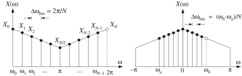
Fig. 9.2.2 N -point DFTs over [0, 2\pi) and over subinterval [\omega_a, \omega_b) , for N = 10 .
