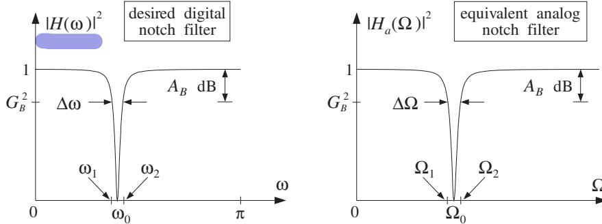
Fig. 11.3.1 Digital notch filter and its analog equivalent.
