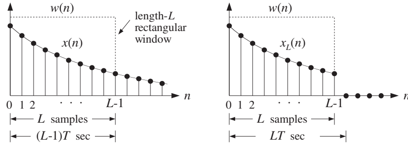
Fig. 9.1.1 Time windowing.
