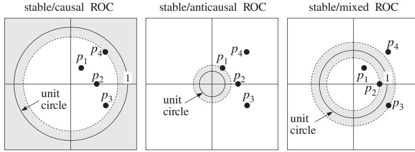
Fig. 5.3.2 Stable ROCs.
