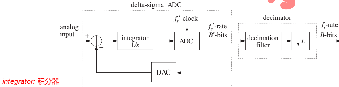
Fig. 12.7.1 Oversampled first-order delta-sigma A/D converter.
