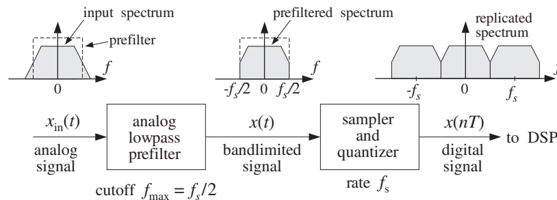
Fig. 1.3.5 Antialiasing prefilter.
