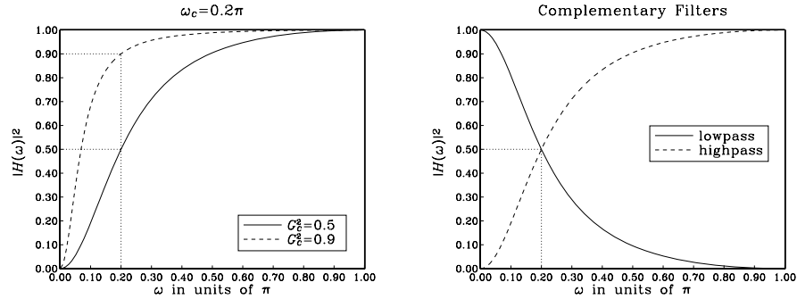
Fig. 11.2.5 Highpass and complementary lowpass digital filters.
