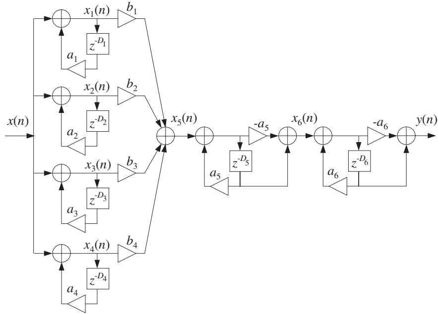
Fig. 8.2.18 Schroeder's reverb processor.
