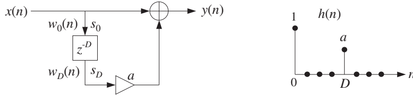
Fig. 8.2.2 Digital echo processor.
