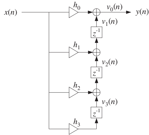
Fig. 4.3.1 Transposed realization of third-order filter.
