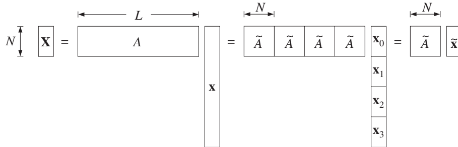
Fig. 9.5.3 N -point DFTs of the full and wrapped signals are equal.
