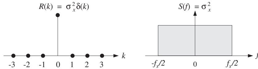
Fig. A.1 Autocorrelation and power spectrum of white noise.
