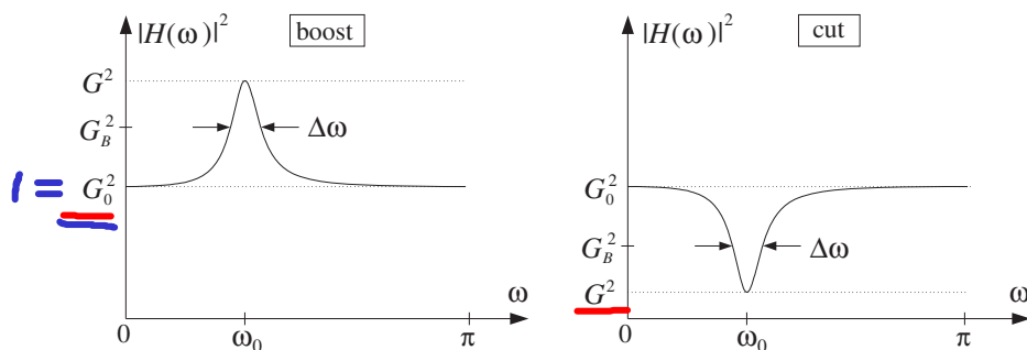
Fig. 11.4.1 Parametric EQ filter with boost or cut.
