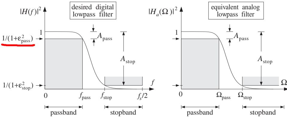
Fig. 11.6.1 Lowpass digital filter and its analog equivalent.
