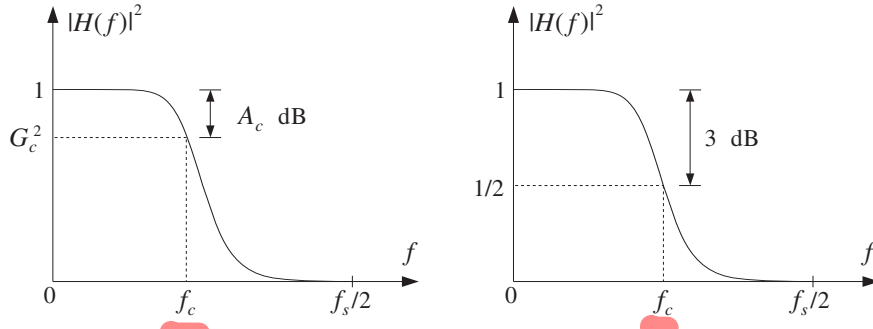
Fig. 11.2.1 Cutoff frequency specifications for lowpass digital filter.
