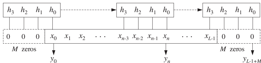
Fig. 4.1.4 Flip-and-slide form of convolution.
