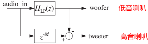
Fig. 10.2.7 Complementary implementation of two-way crossover filters.
