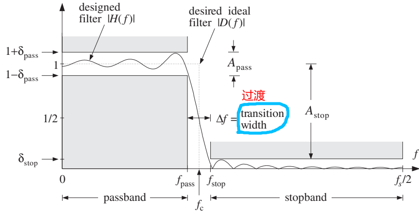
Fig. 10.2.1 Magnitude response specifications for a lowpass filter.
