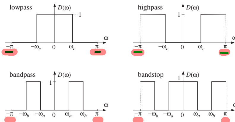
Fig. 10.1.1 Ideal lowpass, highpass, bandpass, and bandstop filters.
