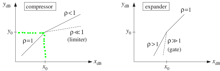
Fig. 8.2.31 Input/output relationship of compressor or expander.
