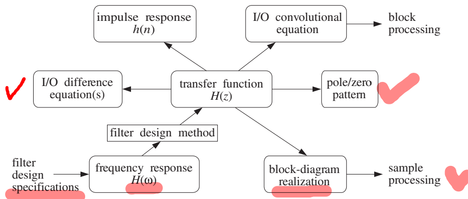
Fig. 6.1.1 Equivalent descriptions of digital filters.
