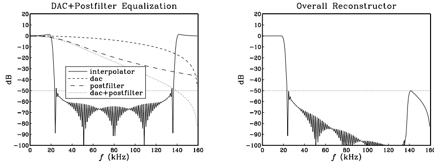
Fig. 12.4.23 4-fold interpolator with equalization of DAC and Bessel postfilter.
