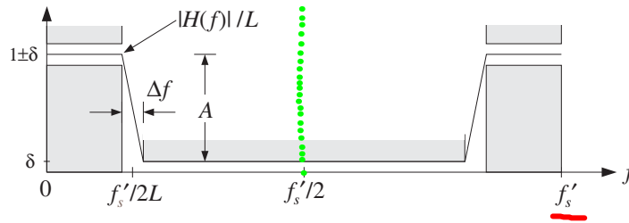
Fig. 12.2.7 Kaiser design specifications for L -fold interpolation filter.
