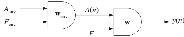
Fig. 8.1.19 Amplitude modulation.
