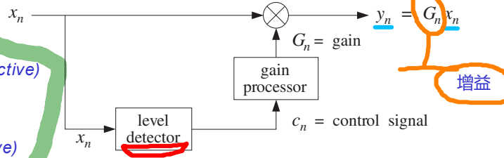
Fig. 8.2.32 Compressor/expander dynamics processor.
