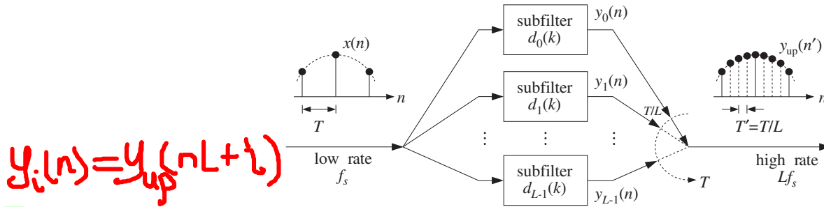
Fig. 12.2.5 Polyphase subfilter implementation of digital interpolator.
