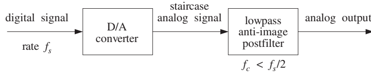
Fig. 12.1.4 Analog reconstruction of sampled signal.
