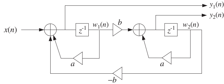
Fig. 8.1.5 Coupled form sine/cosine generator.
