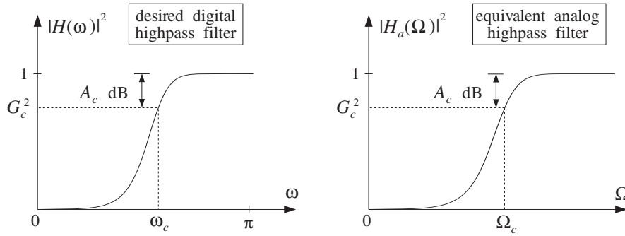
Fig. 11.2.4 Equivalent cutoff specifications of highpass digital and analog filters.
