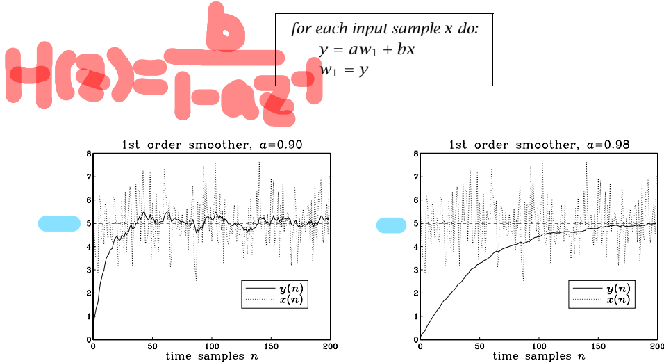
Fig. 8.3.4 Noisy input and smoothed output for Example 8.3.1.
