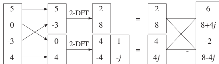
Fig. 9.8.6 4-point FFT of Example 9.8.1.
