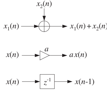
Fig. 4.2.1 Basic building blocks of DSP systems.
