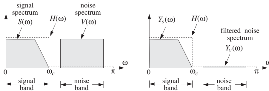
Fig. 8.3.1 Signal and noise spectra before and after filtering.
