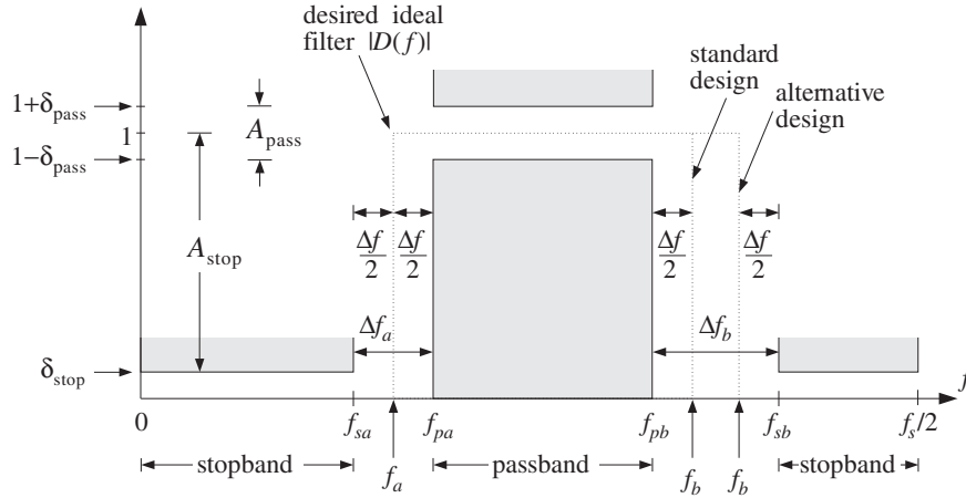
Fig. 10.2.3 Bandpass filter specifications.
