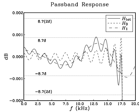
Fig. 12.4.15 Magnified passband of 2×2 interpolator.
