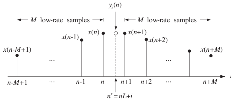
Fig. 12.2.4 Interpolator uses M low-rate samples before and after y_{up}(nL + i) .
