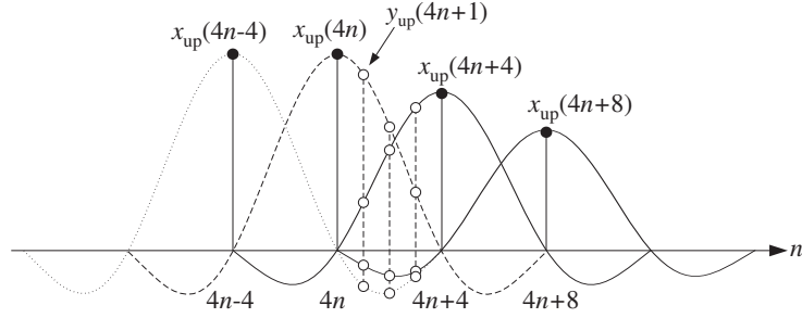
Fig. 12.4.2 LTI form of convolution by superposition of FIR impulse responses.
