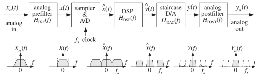
Fig. 1.7.1 Components of typical DSP system.
